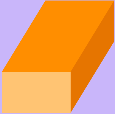
PRISMA RECTANGULAR
