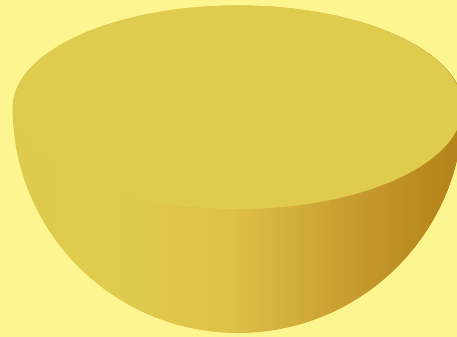
SEMIESFERA
