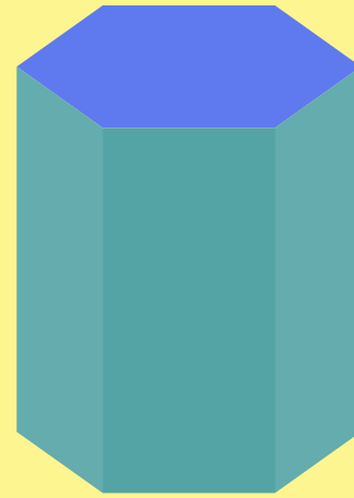
PRISMA HEXAGONAL
