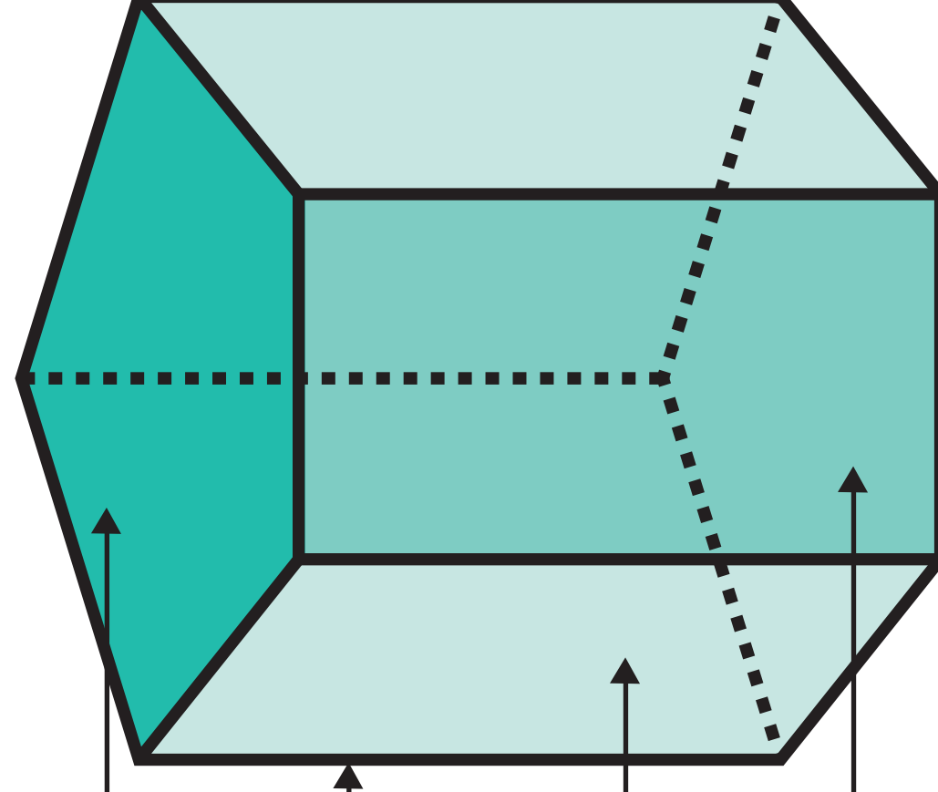
PRISMA PENTAGONAL
